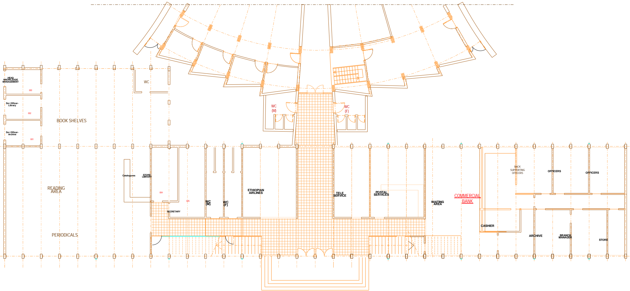
BUILDING- B GROUND FLOOR PLAN 100 m2
