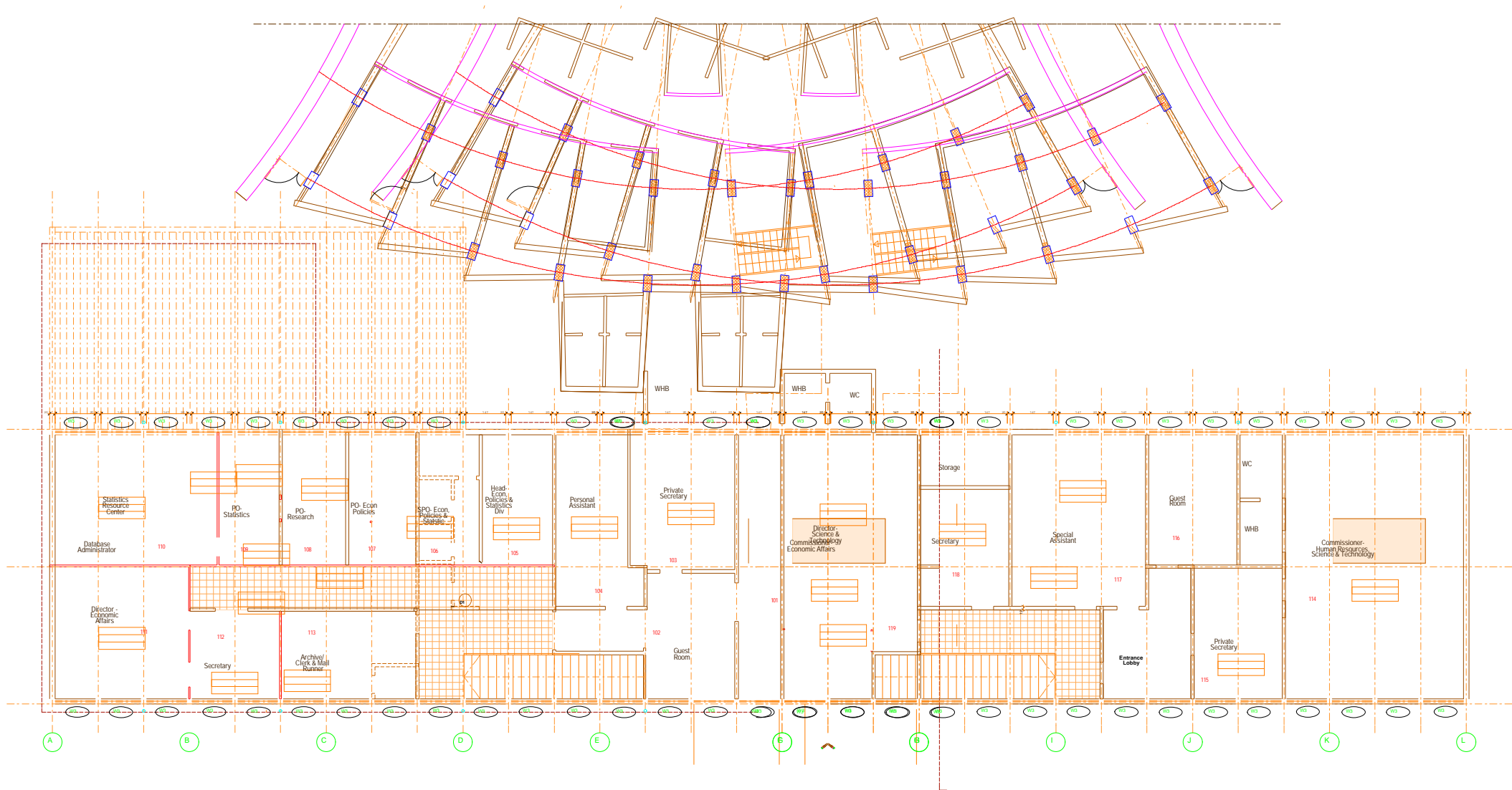
BUILDING- B FIRST FLOOR PLAN 50m2
